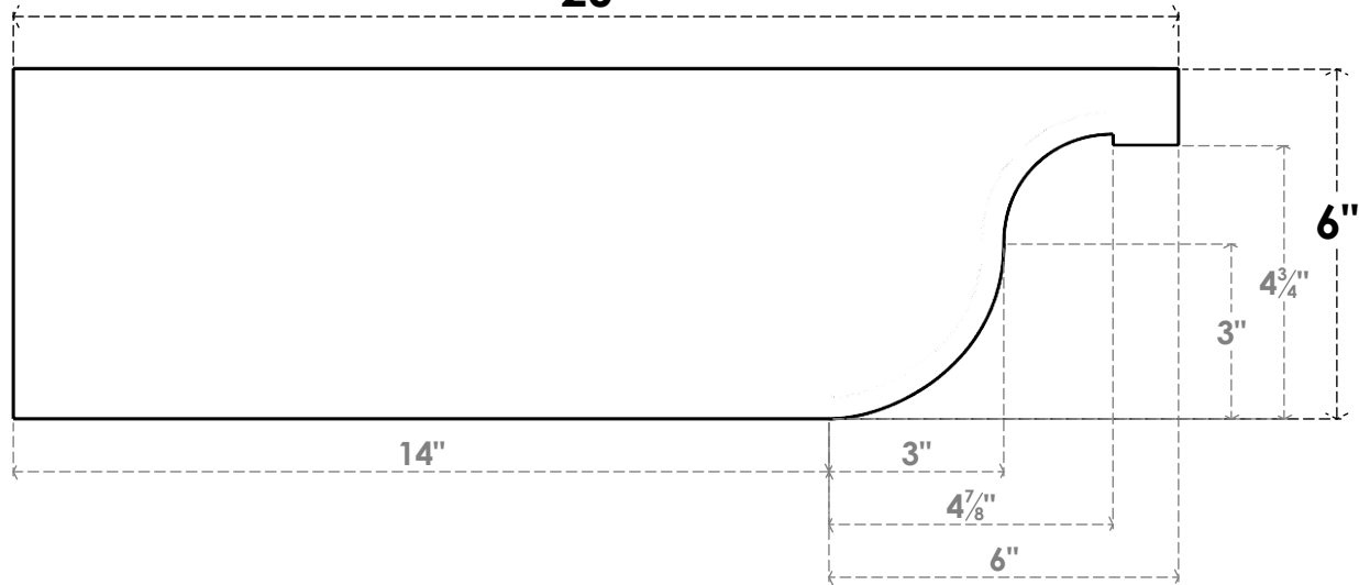
SIDE PROFILE
